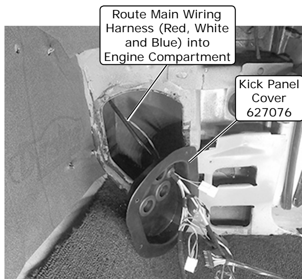
Passenger Compartment View
